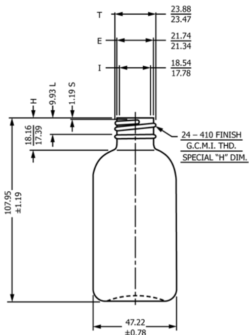
FIG. 1 Standard Container for Permeability Test
